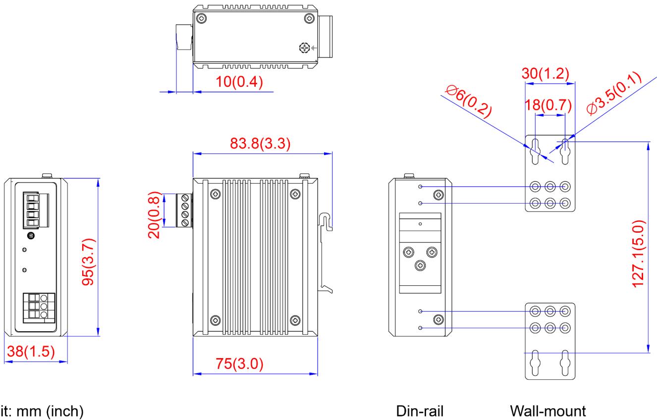
Figure 2.1 - Physical Dimensions
